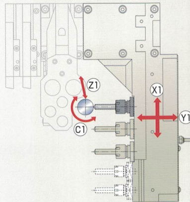
Cross hole ID chamfering
